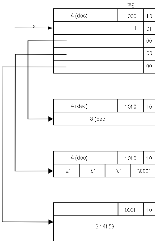
Figure 7-2. The Layout of a Record.
