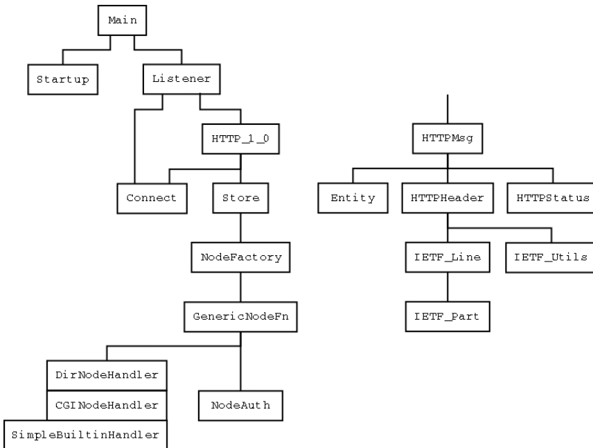
Figure 9-1. The Main Dependencies of the Upper Layers.
