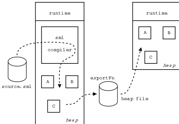
Figure 2-1. Compiling and Running a Program
