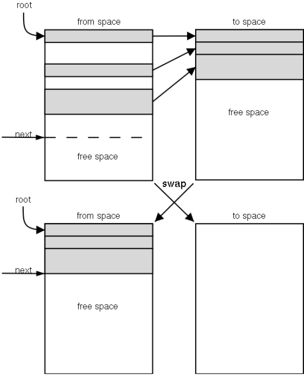
Figure 7-1. Steps in Copying Collection.
