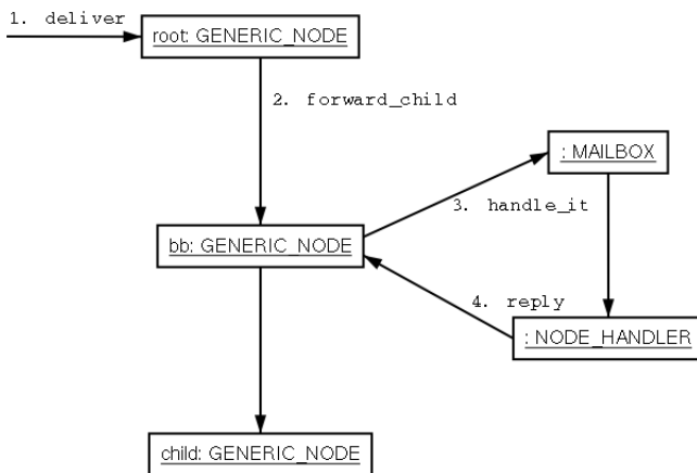
Figure 8-5. A Resource Store Node.
