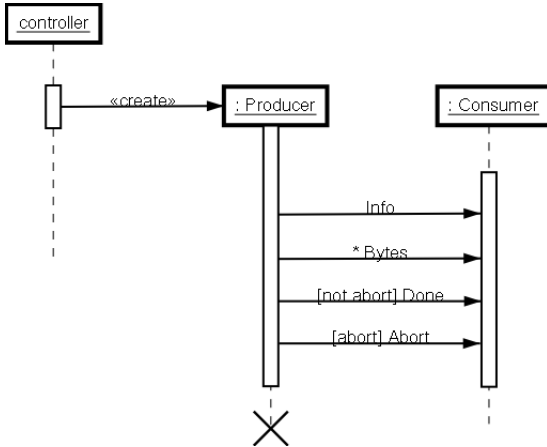
Figure 8-4. The Producer-Consumer Transfer Protocol.
