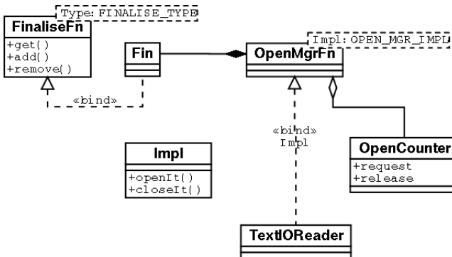
Figure 9-2. The Open Manager Objects.
