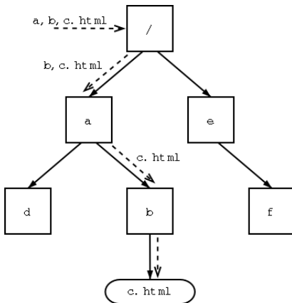
Figure 8-1. A URL navigating the Resource Store.
