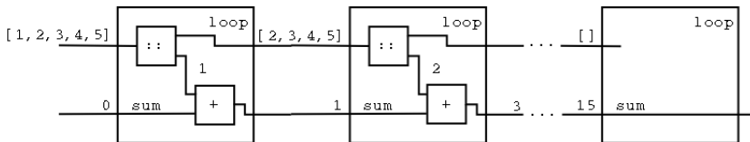
Figure 2-3. Tail Recursion as Data Flow
