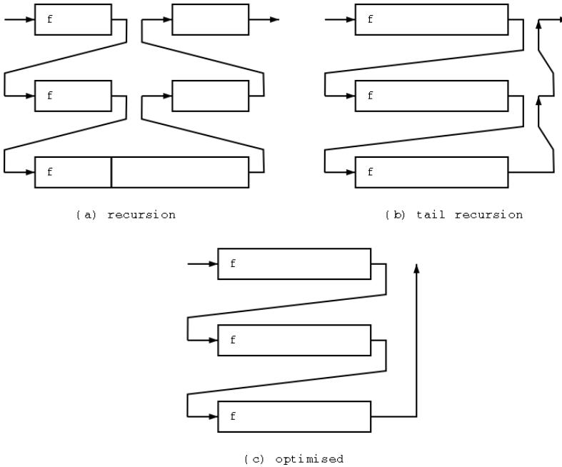
Figure 2-4. Tail Recursion as Iteration
