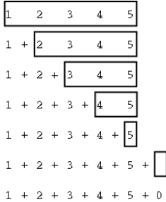
Figure 2-2. Summing a list by Divide and Conquer.
