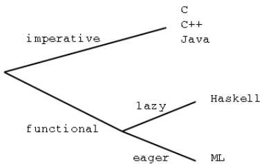
Figure 1-1. A Classification of Some Languages
