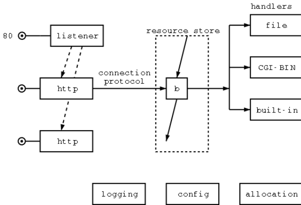
Figure 8-2. The Functional Blocks of the Server.
