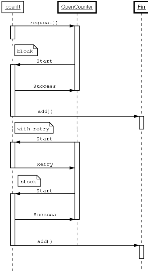
Figure 9-3. The File Opening Handshake.
