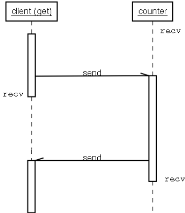
Figure 6-5. Getting the Counter's Value
