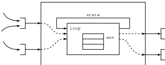
Figure 6-3. A CML Thread
