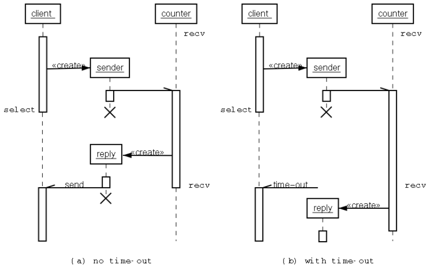
Figure 6-6. Getting the Value with a Time-Out
