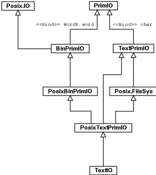
Figure 3-3. The Major Structures Implementing the Portable I/O API
