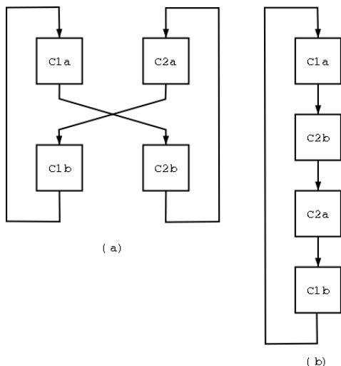
Figure 6-2. Two Coroutines
