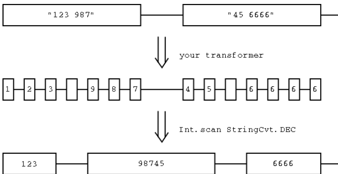
Figure 3-1. Some Stream Transformations
