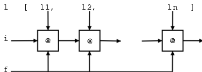
Figure 2-5. The Data Flow for foldl
