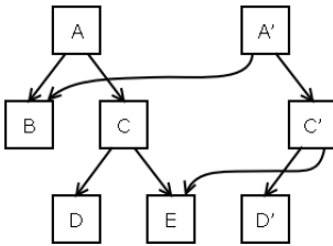
Figure 5-1. Updating a Tree.
