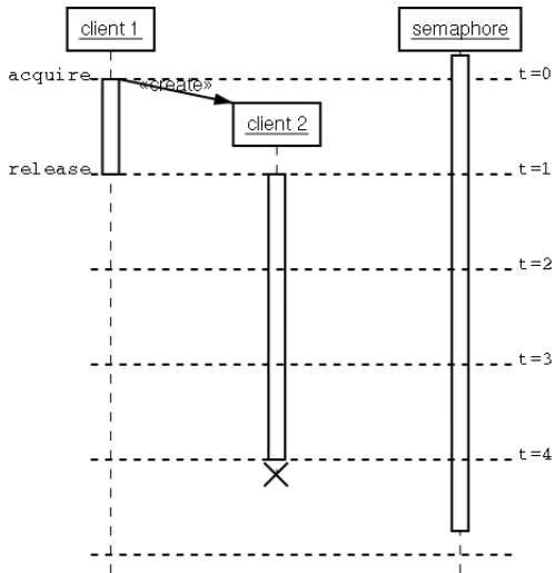
Figure 6-7. The Timing of Semaphore Test 2
