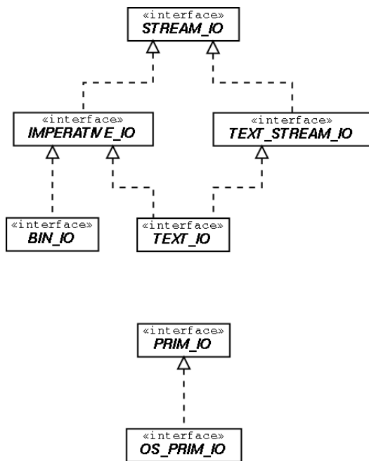
Figure 3-2. The Major Signatures of the Portable I/O API
