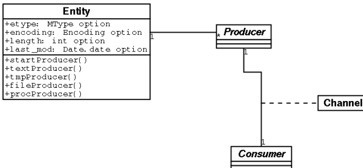
Figure 8-3. Entities, Producers and Consumers.
