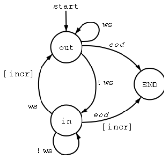
Figure 2-6. Counting Words with a FSM
