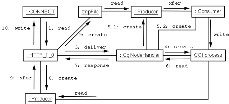
Figure 8-6. Connection-CGI Collaboration.
